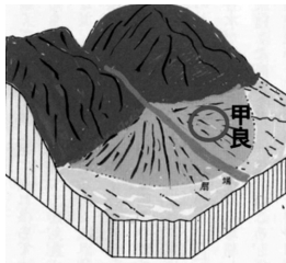
[扇状地模型図]
